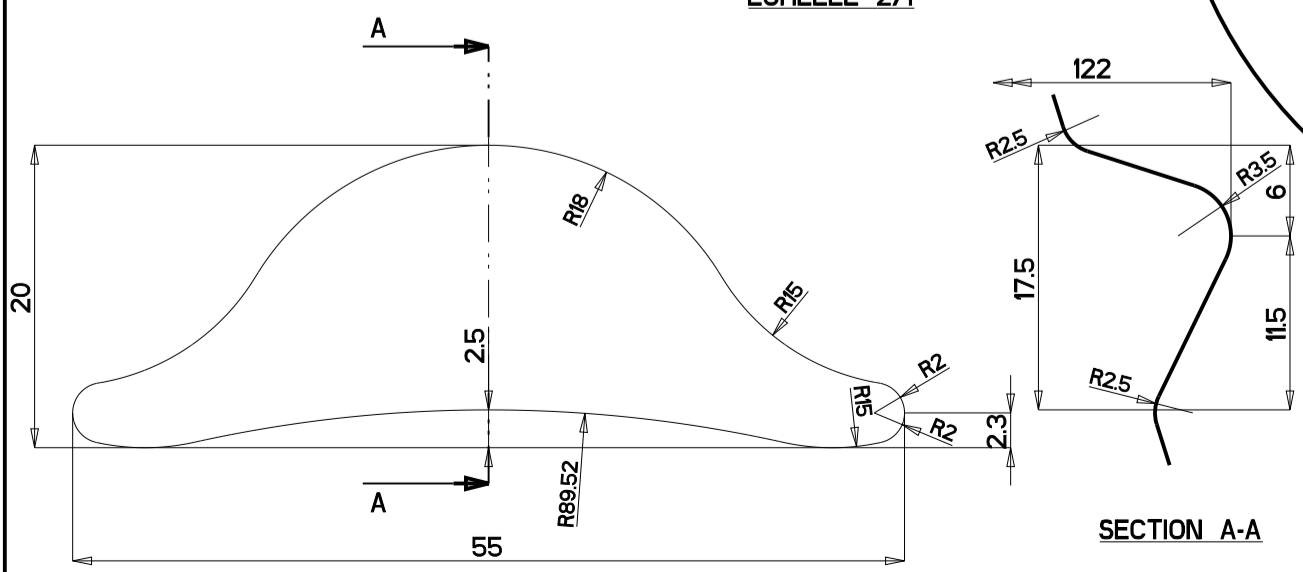
DETAIL ANSE ECHELLE 2/1
